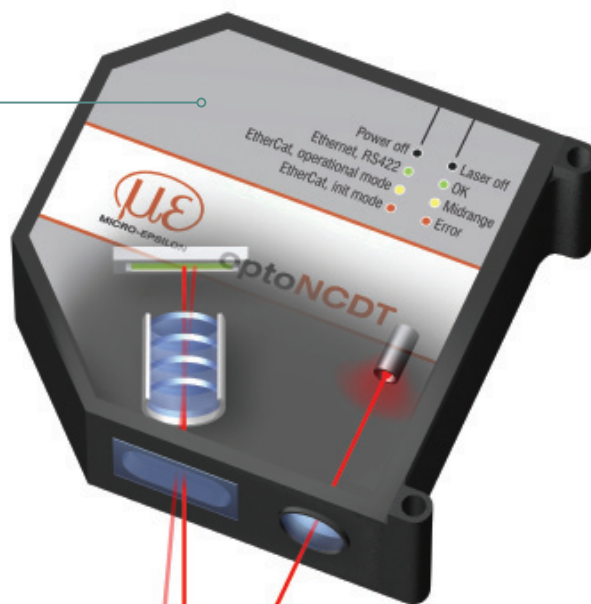
The non-contact displacement sensors optoNCDT utilize optical triangulation as a general measuring principle
