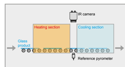
Line scan camera feature measures the temperature distribution between the heating zone and the cooling zone e.g. when toughened or tempered safety glass is heat-treated.
