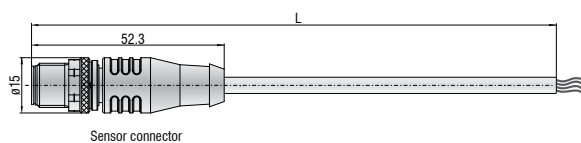
Multi-function cable
