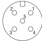
Pin assignment 5-pin M12-connector
